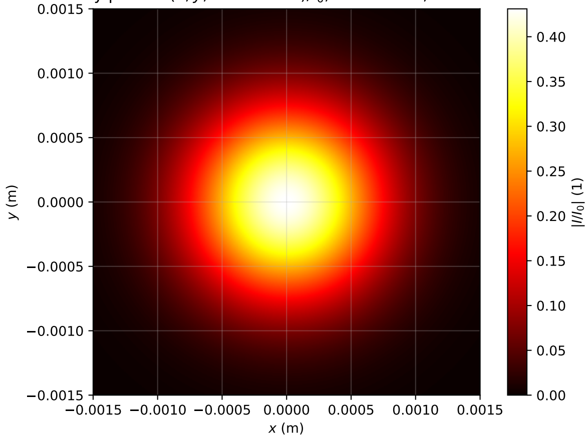
Intensity profile I(x, y, z = 2.468m)/I_0 , P_{in}=0.1P_{cr} , artificial time
